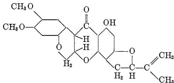
XXIV Sumatrol
