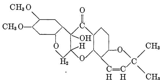
XIV Tephrosin
