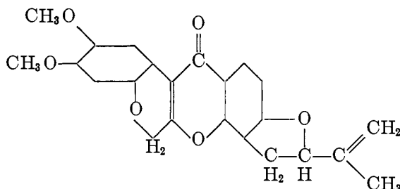
II Dehydrorotenone
