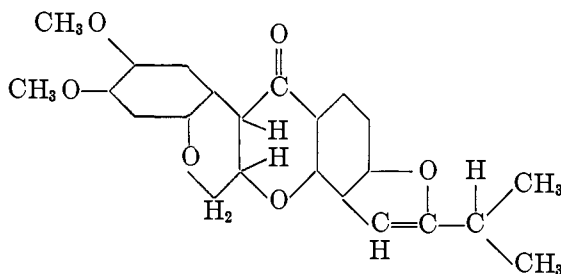
XV Isorotenone
