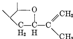
XXIII
